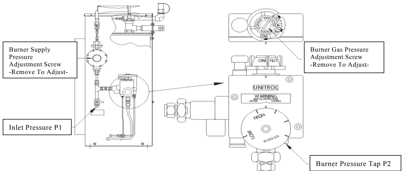
Figure 1. Thermostat pressure points.
